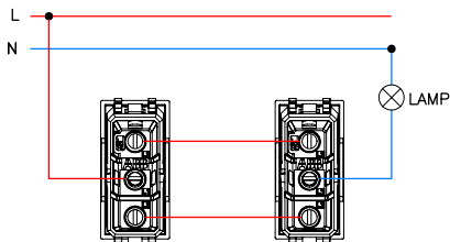
6A 2W switch
