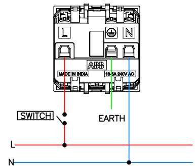
13A Universal socket
